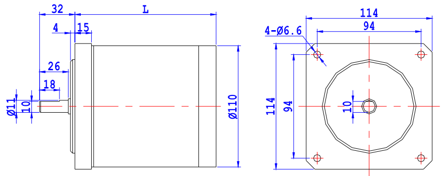
Motor body length can be 115mm, 135mm or 160mm according to different torque.
